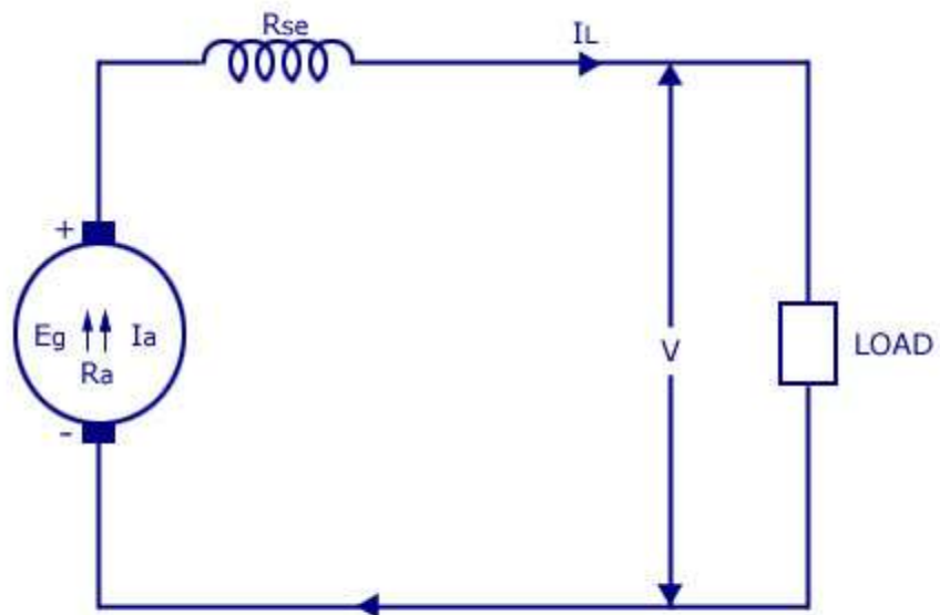
Series (a)
