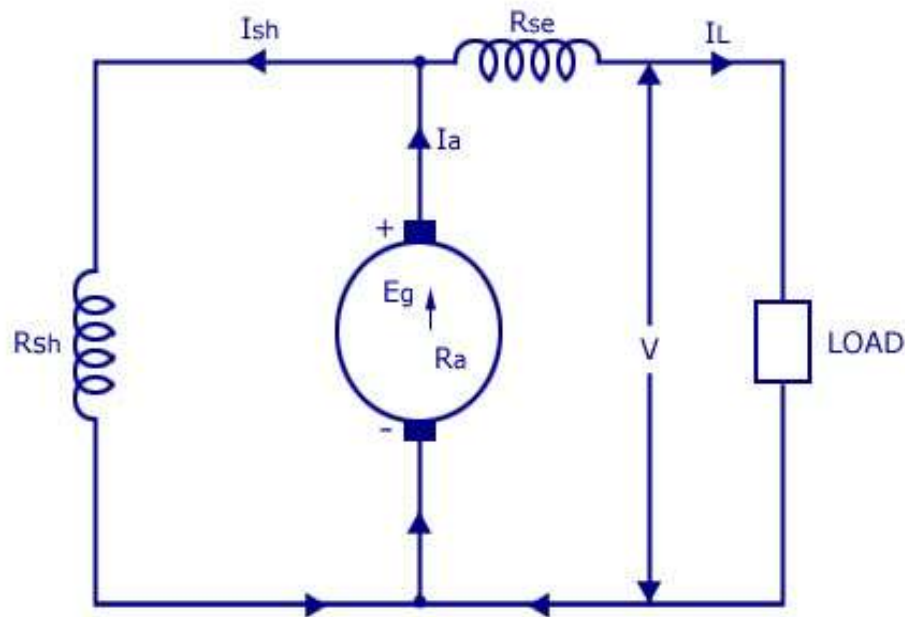
Short Shunt Compound (a)
