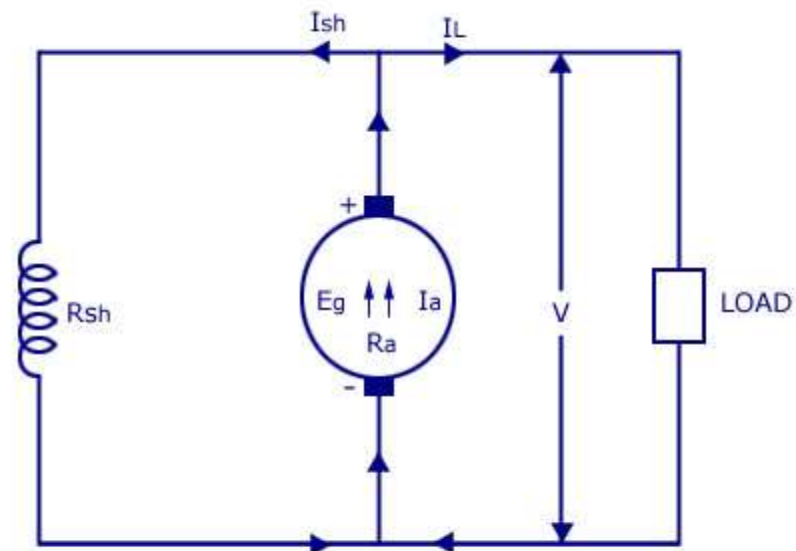
Shunt (b)
